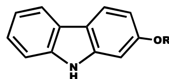
Carbazoles
