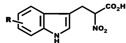
Indole Derivatives
